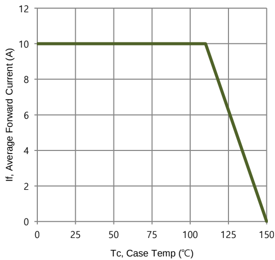
Figure 1 : Current Derating, Case
